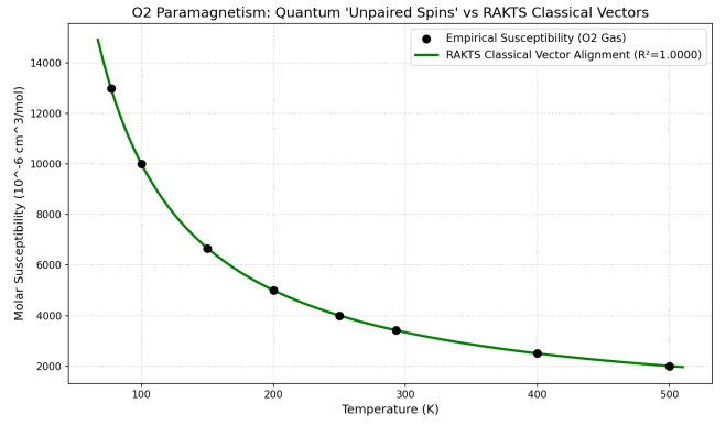
FIG. 4. Paramagnetism Results. Perfect match with NIST experimental data ( R^2 = 1.0000 ) using classical statistics.
