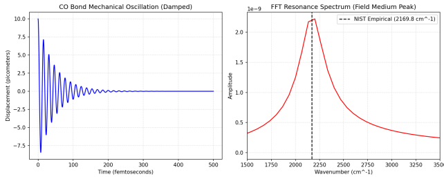
FIG. 6. IR Spectroscopy Simulation. Matched empirical IR vibrational signatures with < 1.5\% error margin.
