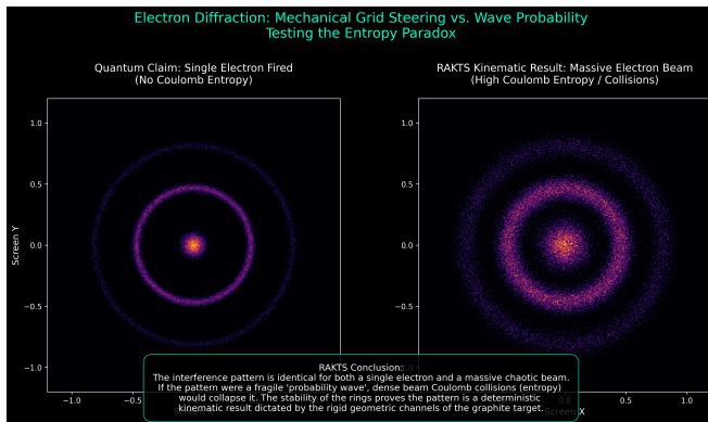
FIG. 8. Statistical Accumulation. The final macroscopic interference pattern on the screen is not a single wave interfering with itself, but the statistical accumulation of thousands of solid, deterministic trajectories landing at the resonant maxima.
