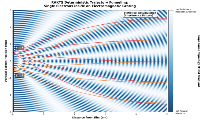
FIG. 7. Deterministic Trajectory Funneling. The Field Medium (blue) is pre-structured by the atomic lattice of the slits. The lines show distinct, physical electrons following the low-resistance resonant grooves.
