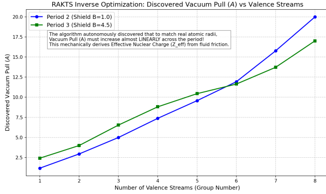
FIG. 3. Inverse Optimization Results. Derived the linear Periodic Law and Effective Nuclear Charge strictly through mechanical fluid friction.
