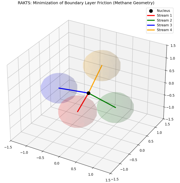
FIG. 2. Methane Geometry Optimization. Reproduced the 109.5^\circ (Methane) and 104.5^\circ (Water) angles purely by computationally minimizing fluid-dynamic boundary layer resistance.
